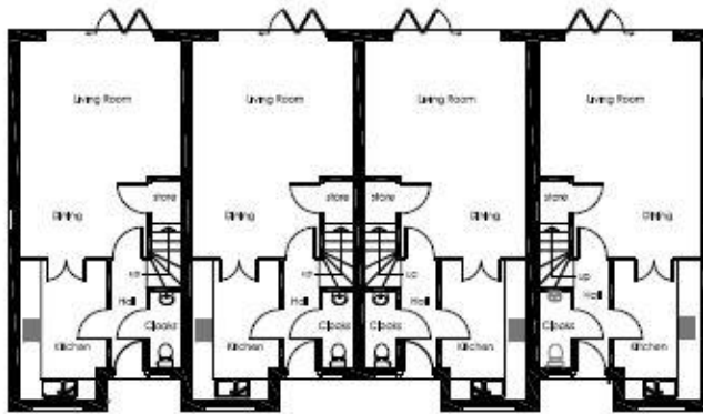
GROUND FLOOR PLANS PLOTS 1-4
