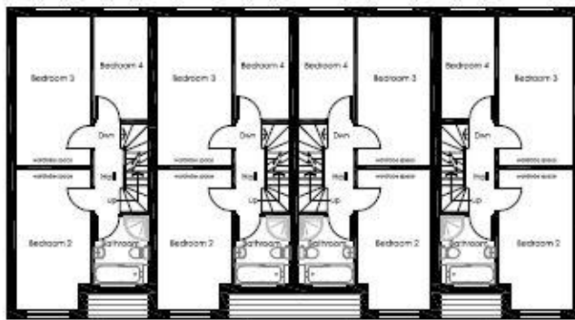
FIRST FLOOR PLANS PLOTS 1-4
