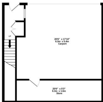
GROUND FLOOR 543 sq.ft. (50.4 sq.m.) approx.
